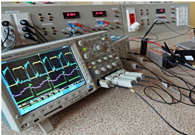
Working place for research and development of new structures for power semiconductor converters
